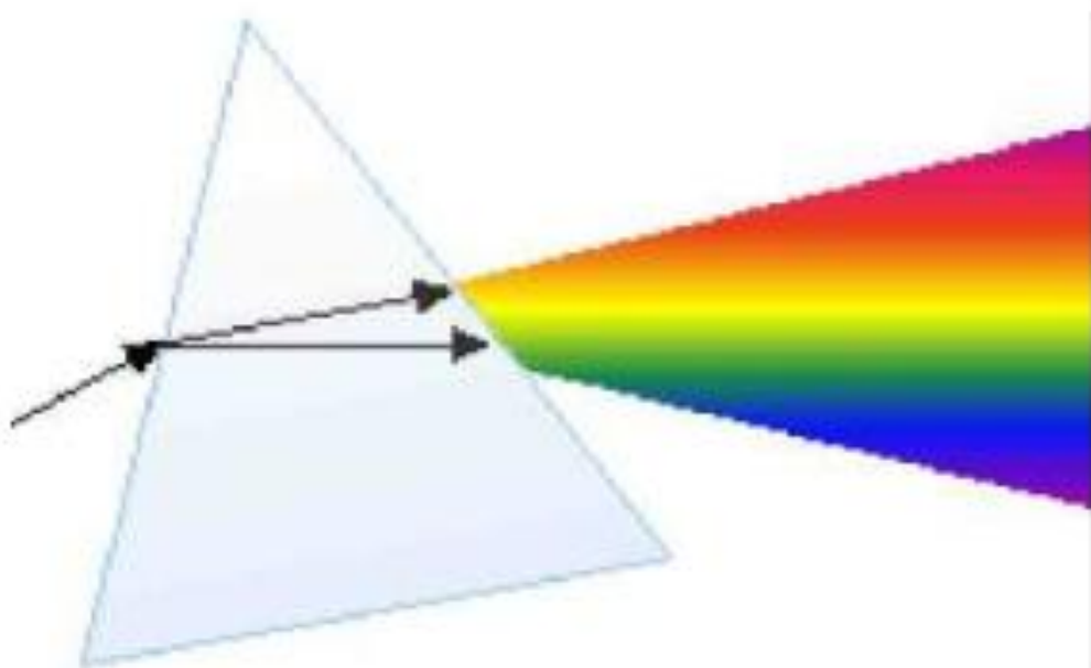
4-rasm Quyosh nurlarining spektrga parchalanishi
